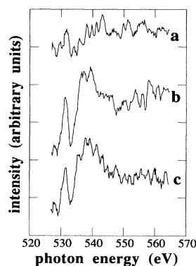
FIG. 2. Oxygen XSEM spectra [2] of a specimen without toxic elements, from three different areas of approximately 2 \times 2 \mu\text{m}^2 : (a) from a substrate area; (b) and (c) from two different axon areas. The two typical optical absorption features of oxygen [13] can be observed at \approx 531 and \approx 538 eV. The data were normalized to the monochromator's output spectrum.
