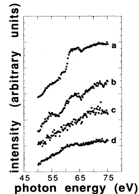
FIG. 3. Cobalt XSEM spectra of (a) a reference Co wire, and from three different 1 \times 1 \mu\text{m}^2 areas of Co-doped specimens; (b) from an axon area and (d) from a cell body in a specimen treated with kainate; (c) from an axon area of a specimen treated with glutamate. The spectra were normalized to the same value for the lowest-energy point and then shifted with respect to each other for clarity. The analysis of the element distribution is discussed in the text.
